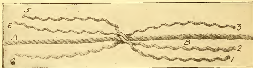
Fig. 9. Starting the Long Splice
